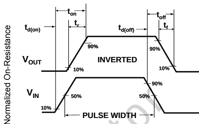
Figure 2: Switching Waveforms
