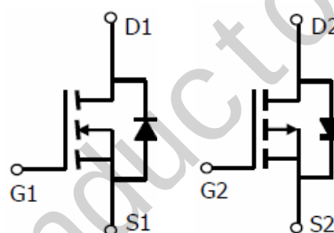
N-channel
